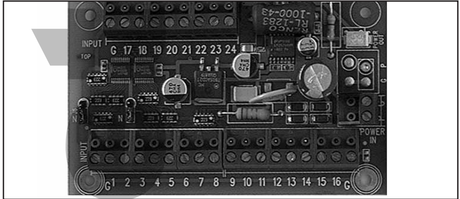
24 Switch Input Connectors on LP-2500 or LP-2600 CPU
