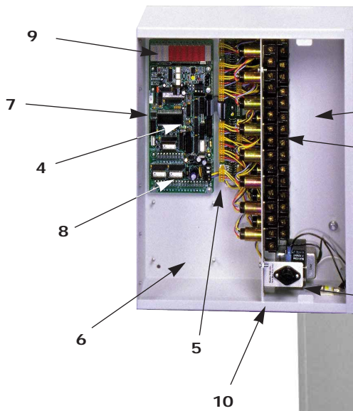
LP-2600 Series
