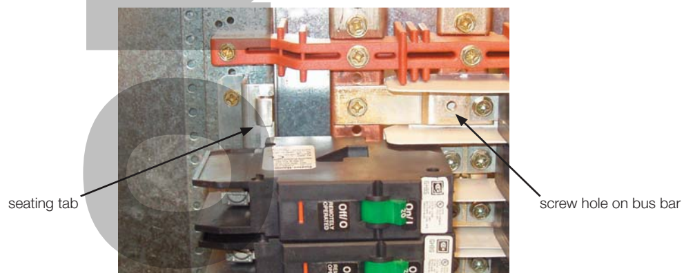
Figure 27 Before adding a new circuit breaker
