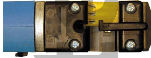
Figure 21a Top view connector loaded
