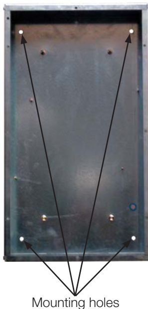
Figure 8 RCS1000 Enclosure
